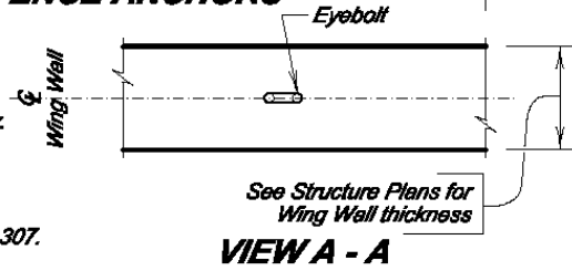
DETAIL FOR FENCE ANCHORS
