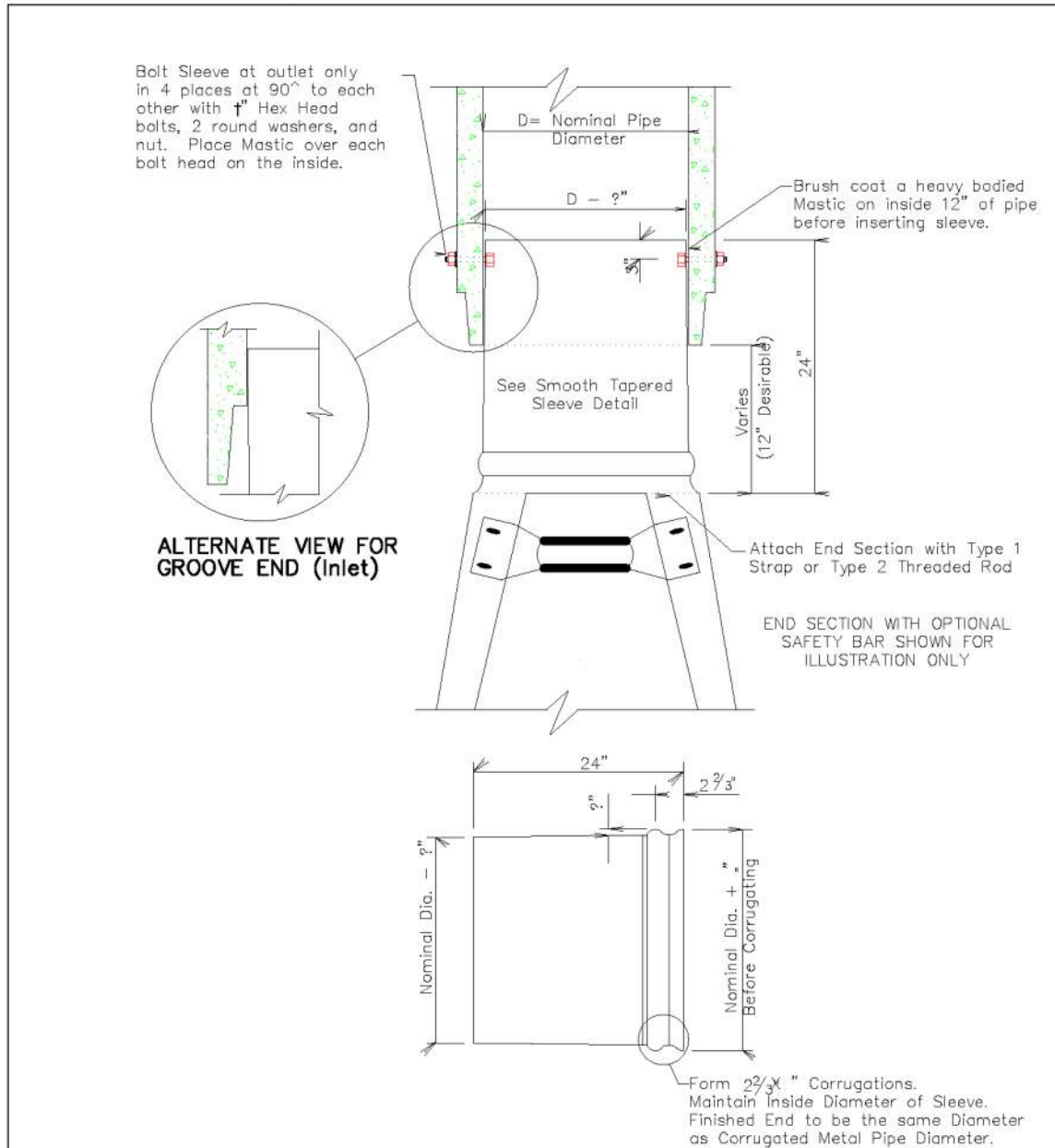
SMOOTH TAPERED SLEEVE DETAIL
