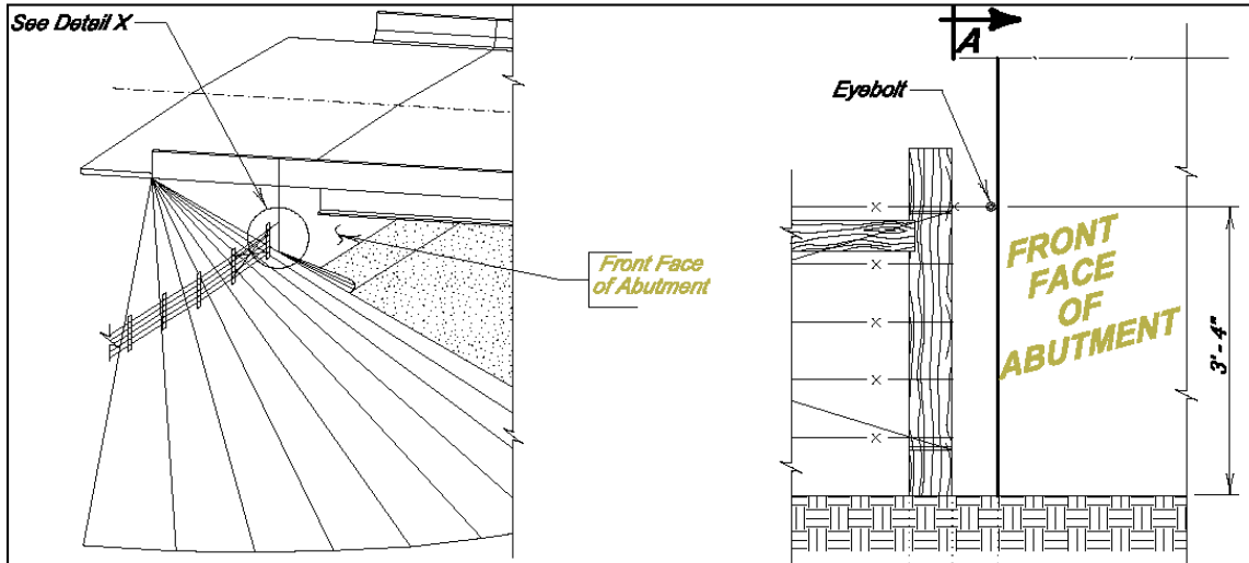
DETAIL "X"
