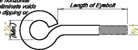
EYEBOLT DETAILS
