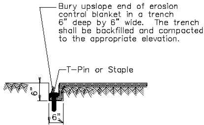
TRENCH DETAIL
