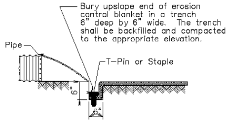
PIPE END DETAIL
