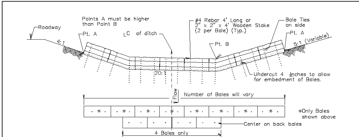
NORMAL DITCH SECTION FOR EROSION BALE INSTALLATION
