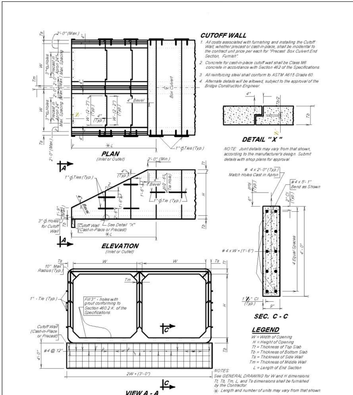
PRECAST DOUBLE BOX CULVERT WITH SLOPED END (4' CUTOFF WALL) NOT TO SCALE
