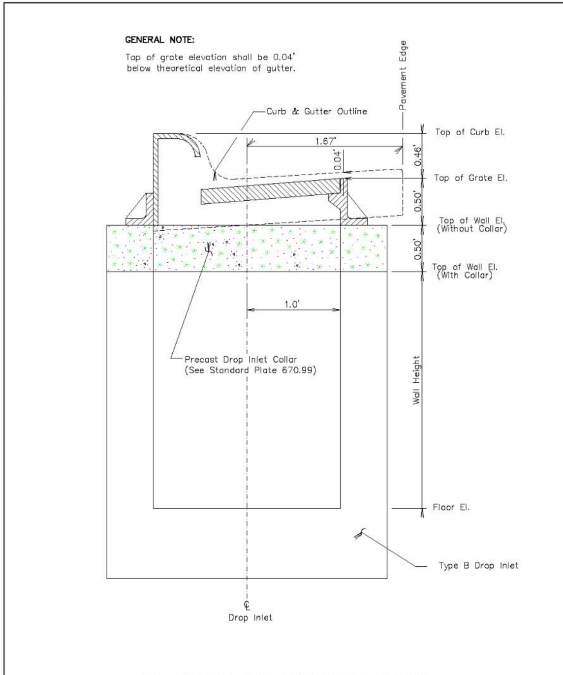
DROP INLET-CONCRETE-TYPE B-INSTALLATION NOT TO SCALE
