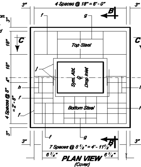
DROP INLETS FOR 12" TO 54" DIAMETER PIPE
