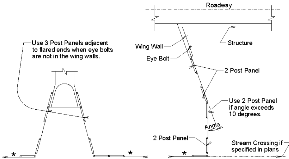
R.C. BOX CULVERT OR CATTLE PASS
